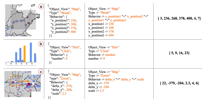
Fig. 2. Examples the encoding process of (a) Brush, (b) Click, and (c) Zoom. These interactions are examples of interactions in Table. 1. They are converted to JSON representations, then to CFG Parsed Tree, and then to numerical vectors based on the rules generated by CFG Tree. the same rule-governed format since the method is conducted over the whole dataset. The parsed-tree consists of the following keys:
