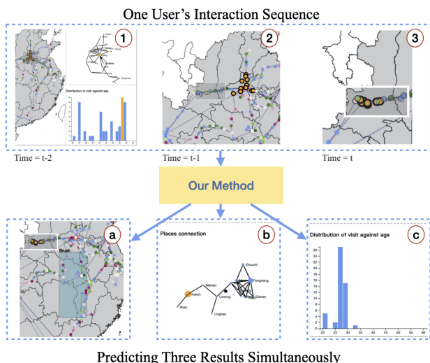
Fig. 6. One example of recommendation results of one input sequence of interaction logs. ①click a column on the Histogram View②brush an area on the Map View③zoom into an area on the Map View, compose a sequence of user interactions and the corresponding visual states. @brush on the Map View @click on the Force-Directed View@click on the Histogram View are the recommendations given by our model.
