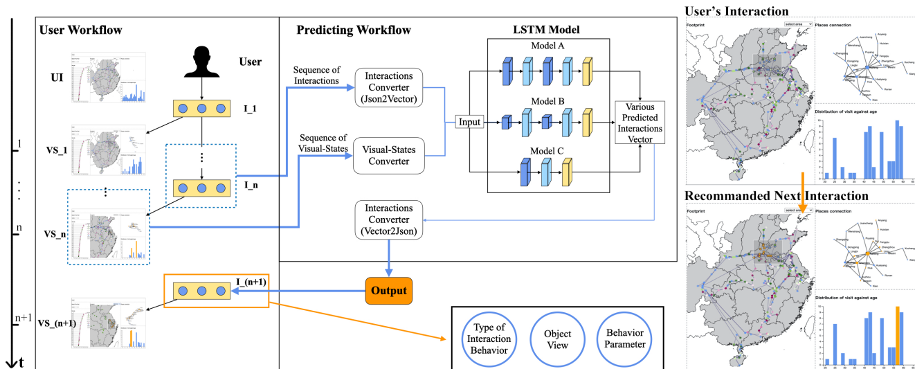
Fig. 1. A high-level illustration of our workflow for recommending interactions. In the user's workflow, each time the user completes an interaction, the system collects the interactions and visual states and then transfers them to the converters in a sequence. In the predicting workflow, the pre-trained LSTM models receive inputs and then output various predicted interaction vectors. After being converted to JSON data, the corresponding recommended interactions will be presented to the user. The two UIs on the right represent one user's interaction of brushing in the Map View, and the system gives the recommended interaction of selecting one column in the Histogram view for the next step.
