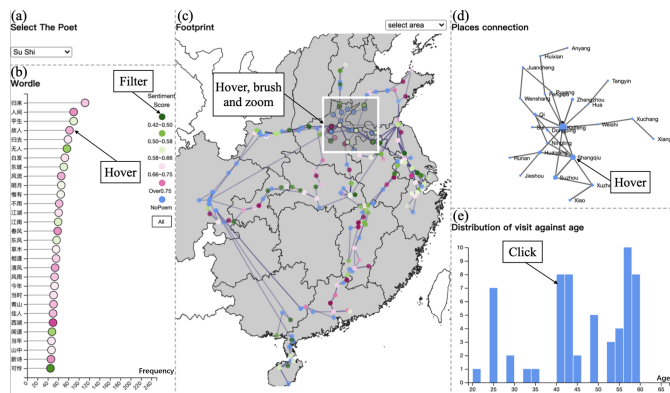
Fig. 5. The Interface of the System. (a) Select one poet to explore. (b) Wordle View. (c) Map View. (d) Force Directed Graph View. (e) Histogram View.
