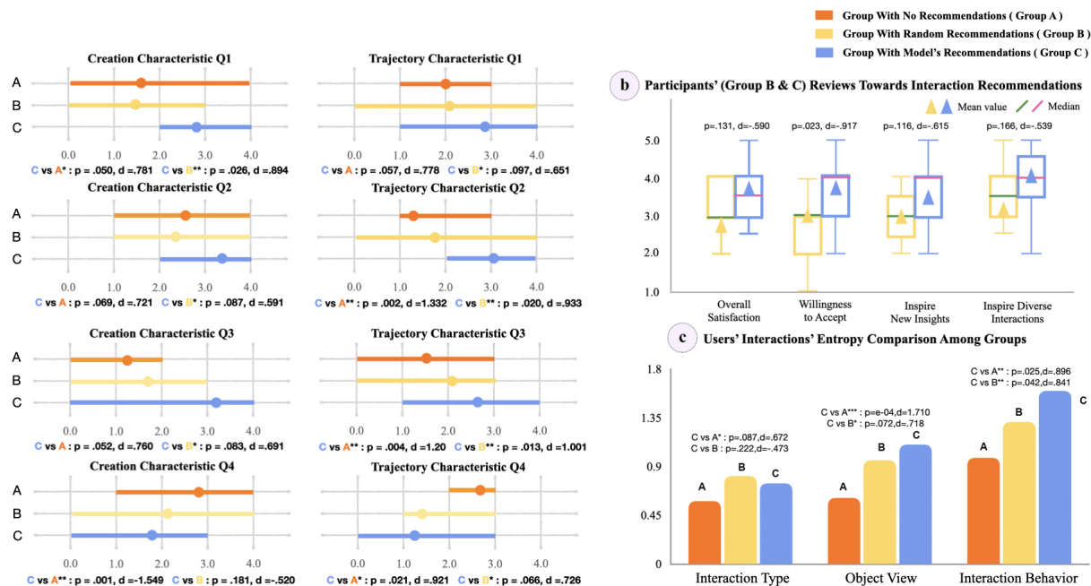
Fig. 7. Data Insights. Questionnaire Rating (a) shows the distribution of the acceptance degree of insight statements, with the results of paired t -tests' p -value between our model and two control groups (*, ** and *** denote p < .05 , .01 and .001 , respectively). The higher degree of acceptance of the correct statement (Creation and Trajectory Characteristic Q1-Q3), the better the data insight obtained by the user. 5-Points Likert Scales (b) shows users' reviews of random recommendations and our model's recommendations. Bar Chart (c) shows user's interactions' entropy in the aspect of interaction types, object views, and interaction behaviors among three different groups, along with the results of t -tests.
