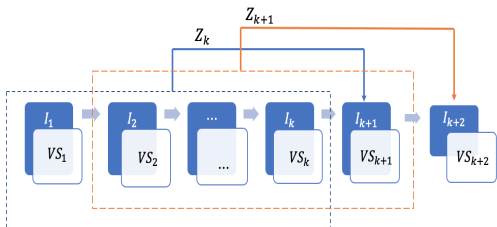
Fig. 3. The Data Structure of LSTM Model. The first k {Interaction, Visual States} are sequenced together to form an input value Z_k , and the corresponding label value is the next interaction I_{k+1}
