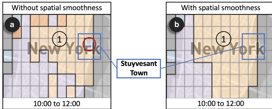
Fig. 8 The analysis results in the map view generated a without and b with the spatial smooth regularization terms
