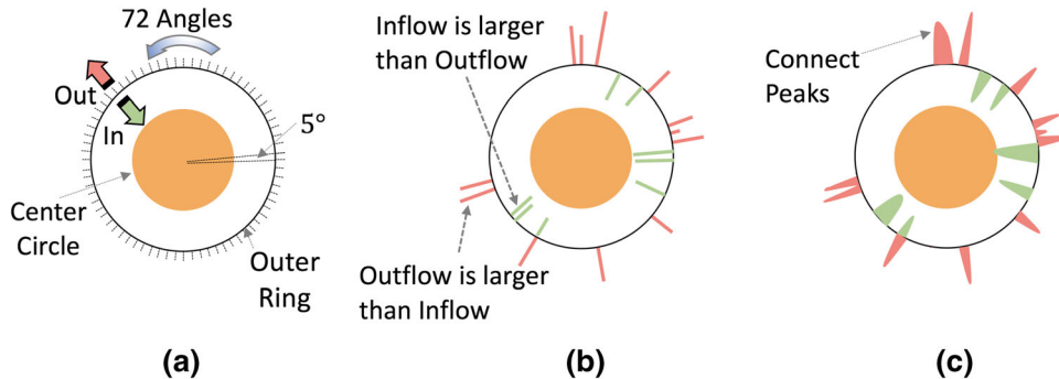
Fig. 5 Flow-glyph design. a The center circle and outer ring, respectively, show the amount and direction of traffic flows in the grid. b These flows are visualized as bars and c enhanced by a colorful peak with red indicates outflow and green indicates inflow
