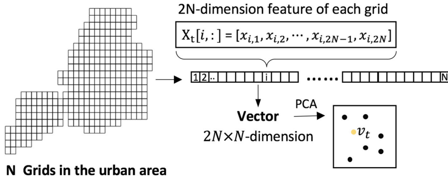
Fig. 4 The characteristic of point v_t is captured by an N \times 2N -dimensional feature vector, where N indicates the number of grids in a region and 2N is the number of features of each grid
