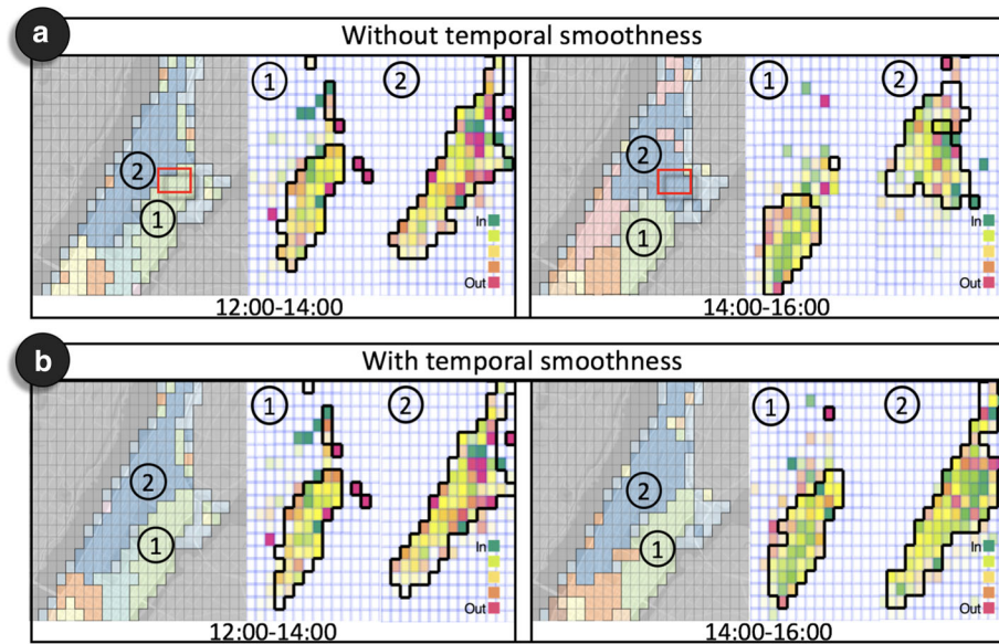
Fig. 7 The analysis results in the map view and pattern view generated a without and b with the temporal smooth regularization terms
