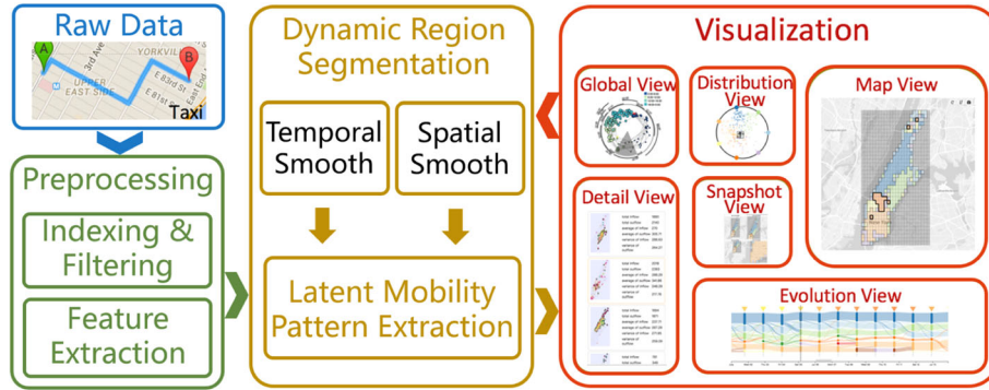
Fig. 1 The system pipeline of EcoLens. Three primary modules, including preprocessing module, analysis module, and visualization module, support the analysis of evolution patterns of latent regions within the urban context
