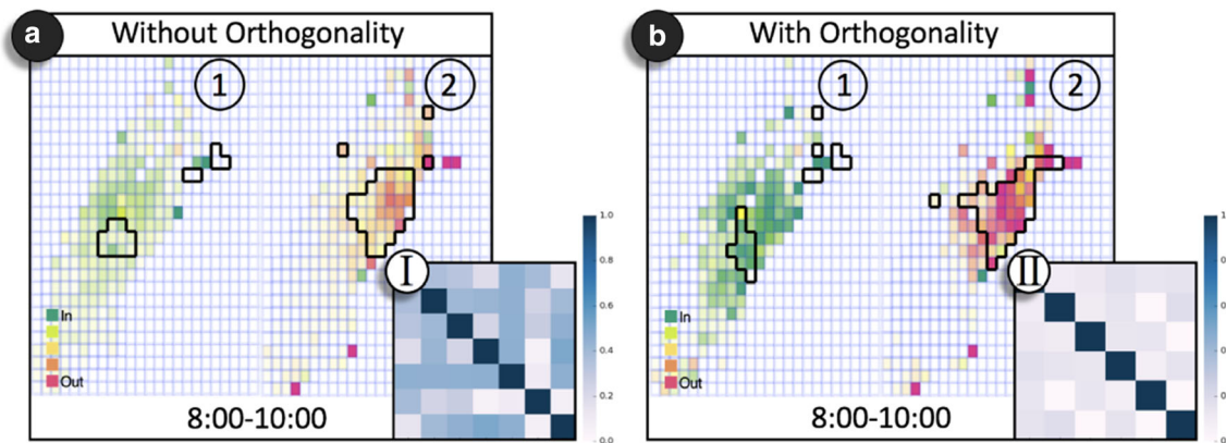
Fig. 9 The analysis results in the pattern view generated a without and b with orthogonality constraint. (I) and (II) show the corresponding correlation matrices of a and b , respectively
