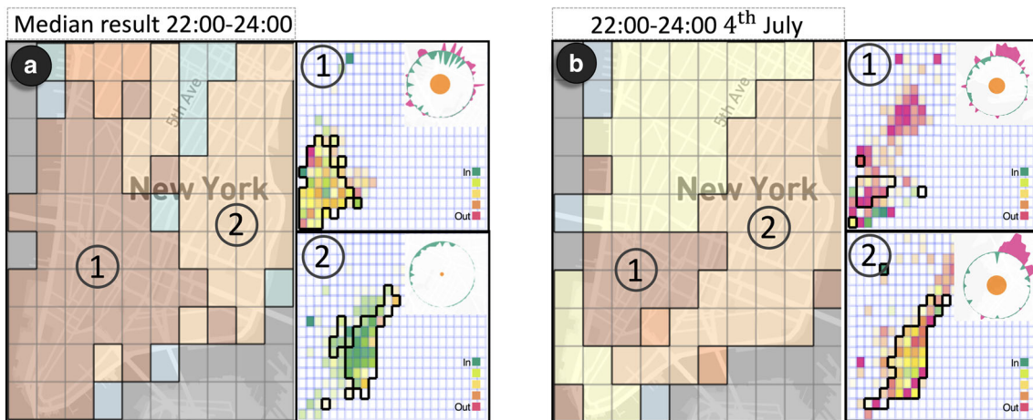
Fig. 12 By comparing to a the normal pattern, b the anomalies traffic flows near the Brooklyn Bridge on July 4th, 2014 (the Independent day) is revealed
