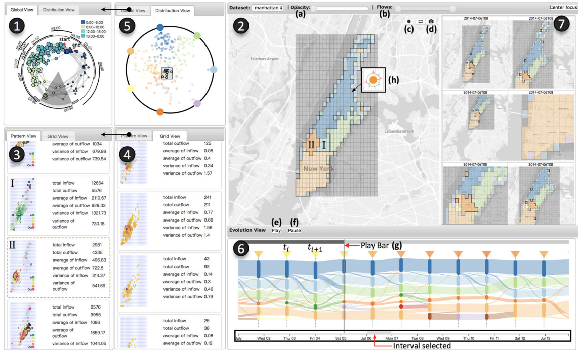
Fig. 3 The user interface of EcoLens consists of seven major views: (1) global view, (2) map view, (3) pattern view, (4) grid view, (5) distribution view, (6) evolution view, and (7) snapshot view
