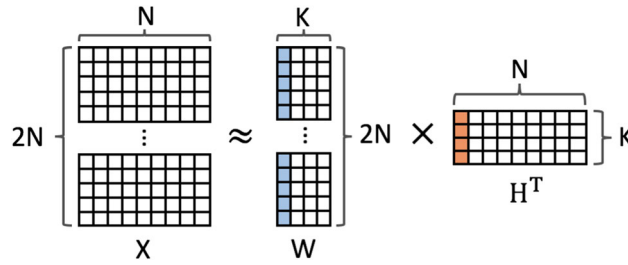
Fig. 2 Matrix X is decomposed into the product of matrix H and W . The column in H^T highlighted in red indicates the likelihood of the K mobility patterns occurred in the 1st regions. The column in W highlighted in blue shows the probability of the 1st mobility pattern having a certain feature
